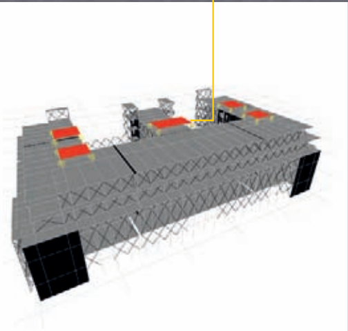
Model of Palatul Victoria with TMCS
