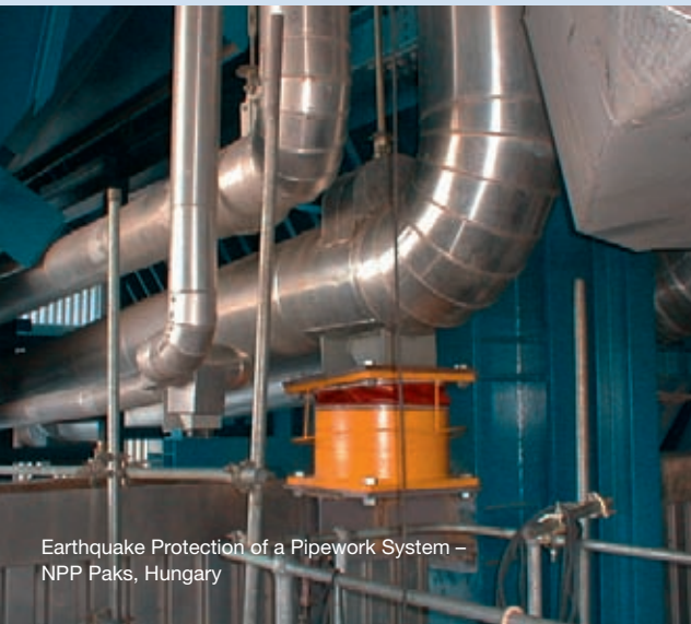
Spring Viscodamper® BCS
